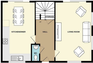
GROUND FLOOR 643 sq.ft. (59.7 sq.m.) approx.
