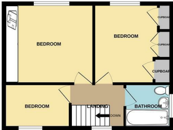
1ST FLOOR 404 sq.ft. (37.5 sq.m.) approx.
